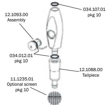
Saliva Ejector Assembly without Tubing 12.1258.00
