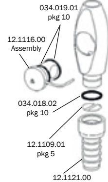
Saliva Ejector Assembly without Tubing 12.1258.00
